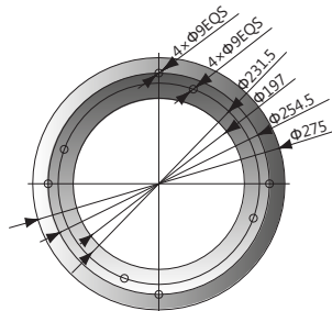
SHR-6U-S~SHR-24U-ST Talp méret
