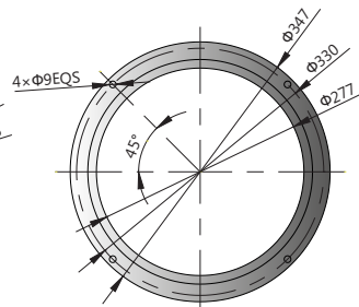
SHR-36U-ST~SHR-48U-ST Talp méret
