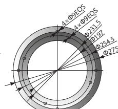
SHR-6U-S~SHR-24U-S Talp méret
