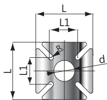
SHR-U-EST talp méret
