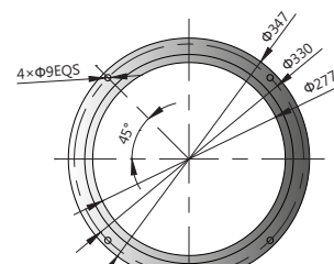
SHR-36U-S~SHR-96U-S Talp méret
